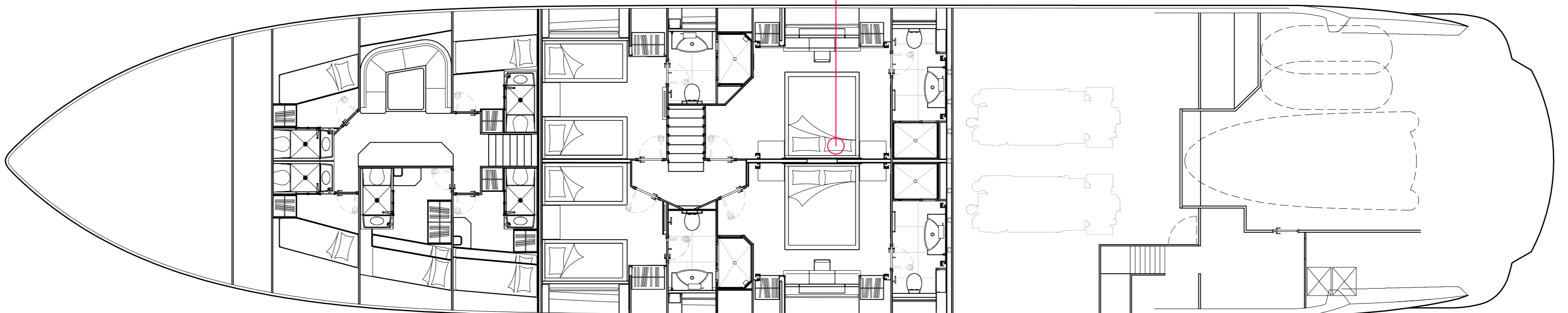
LOWER DECK
