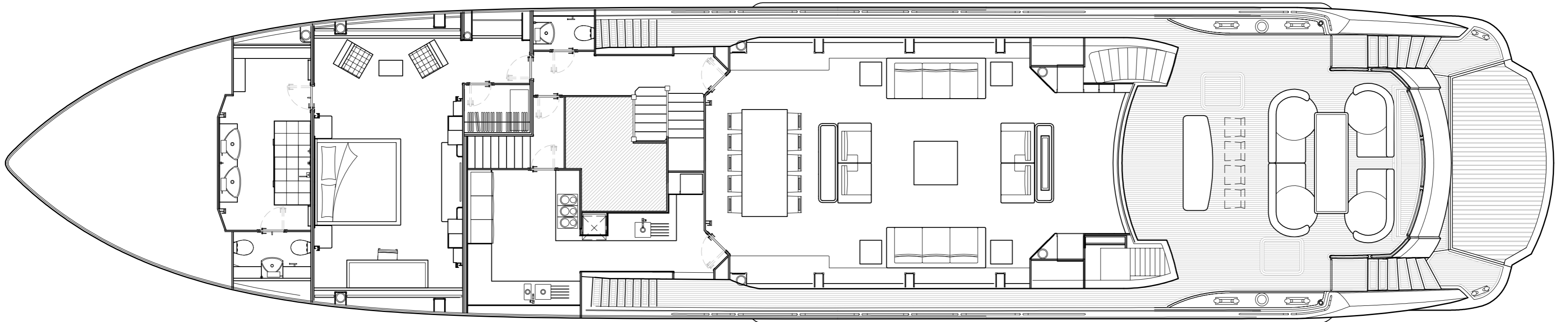
MAIN DECK
