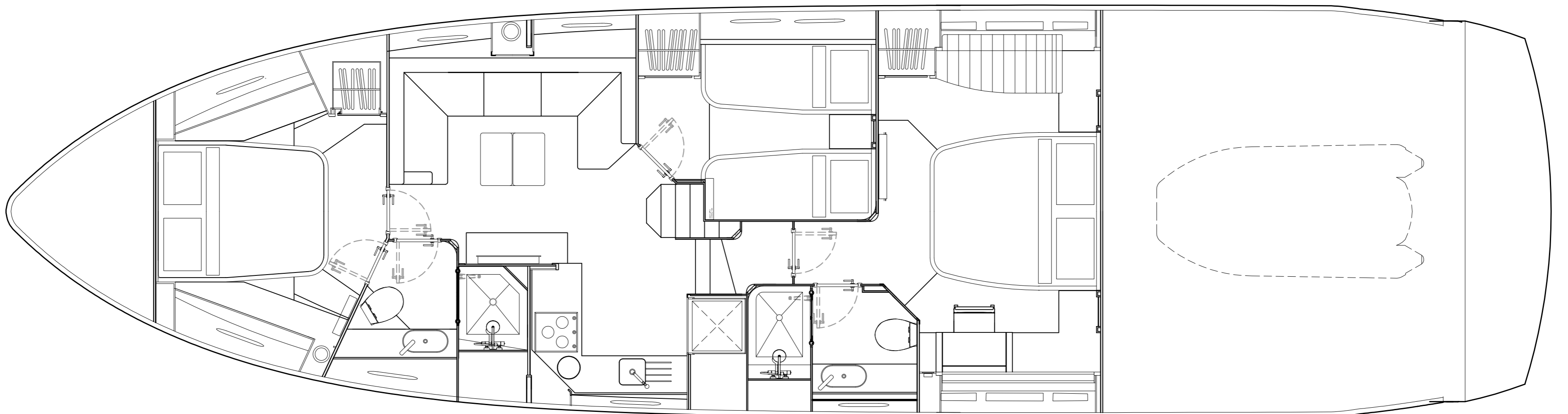
LOWER DECK Shown with tender size to suit open cockpit arrangement
