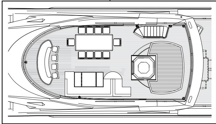
Skydeck option Forward bar area, port side seating, starboard side dining and aft spa tub and sun pad arrangement
