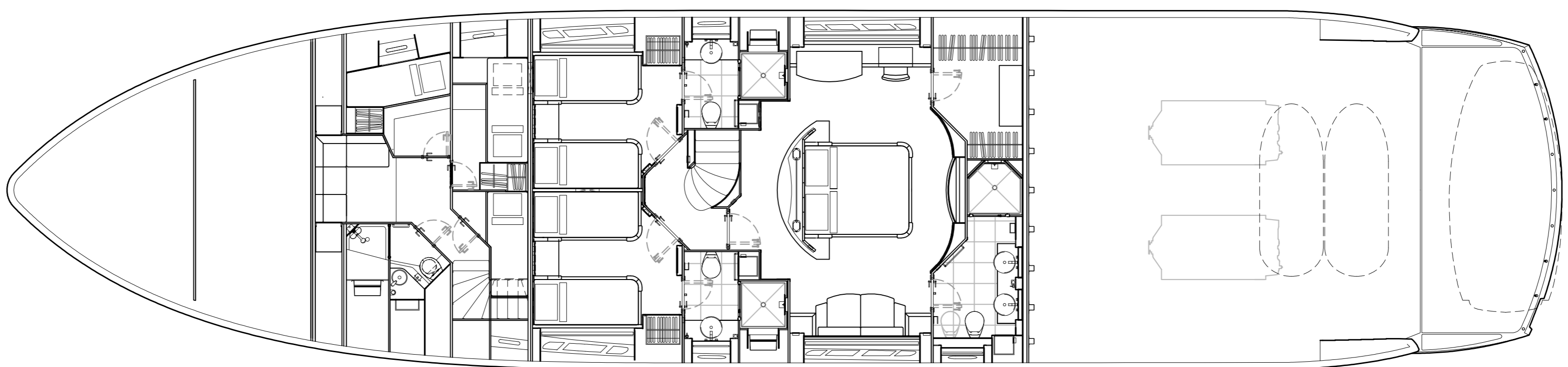
LOWER DECK
