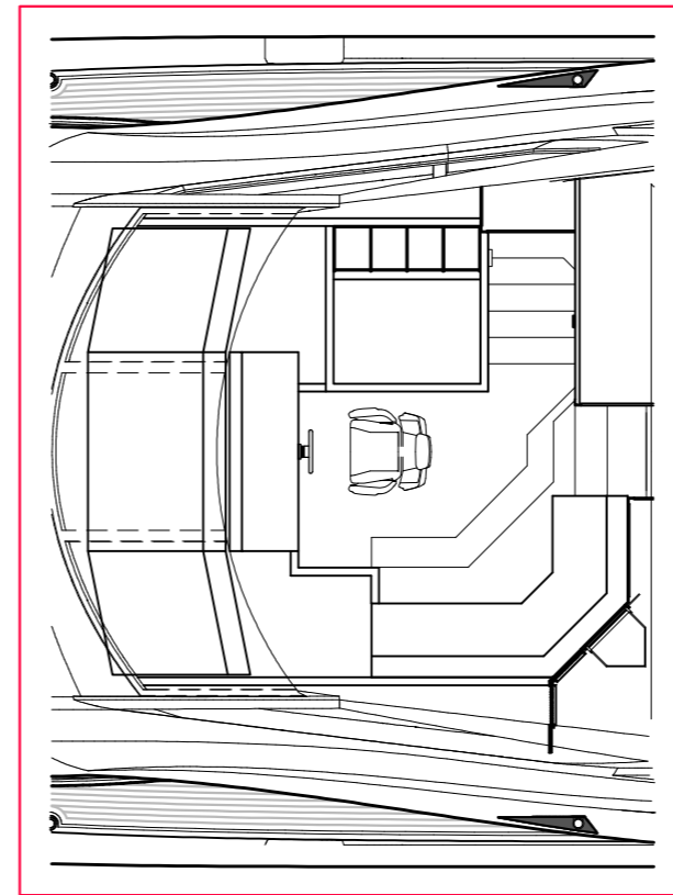
WHEELHOUSE
