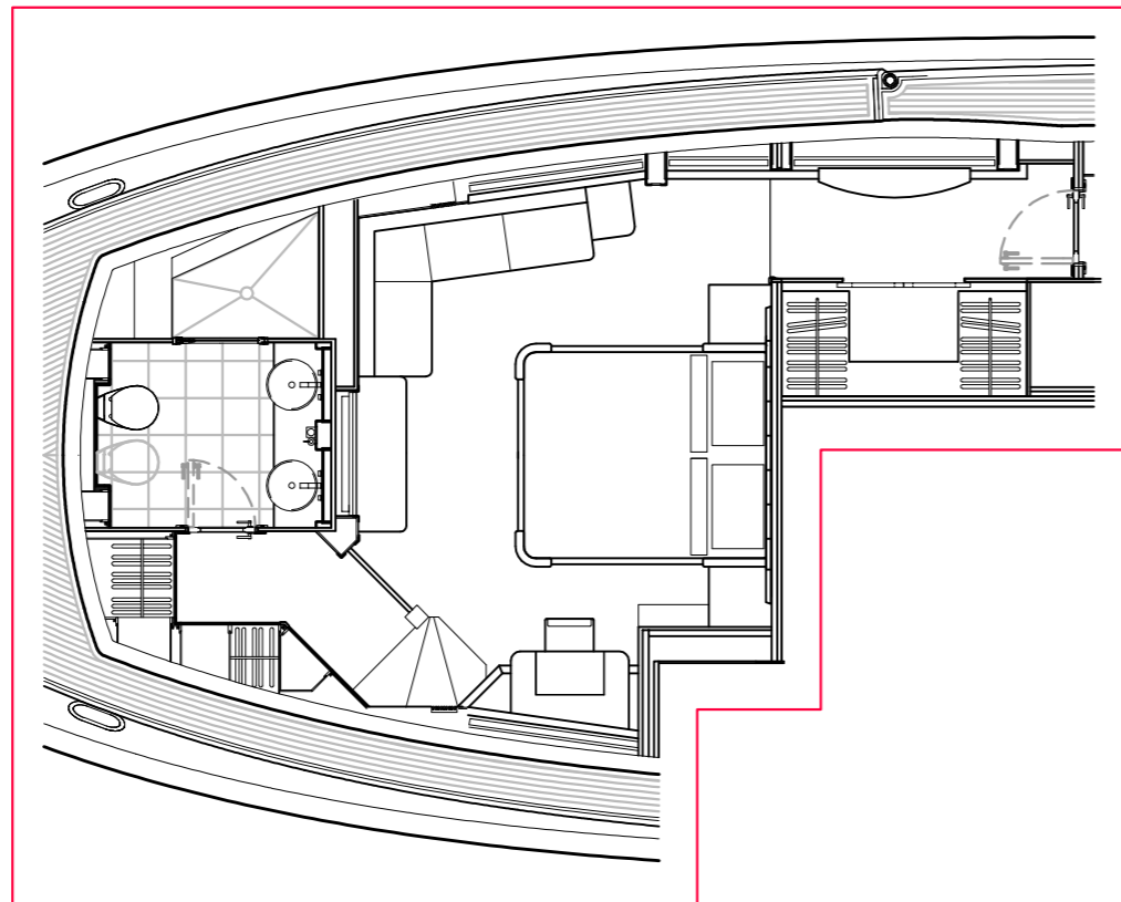
MAIN DECK OPTION; Master stateroom with en suite forward
