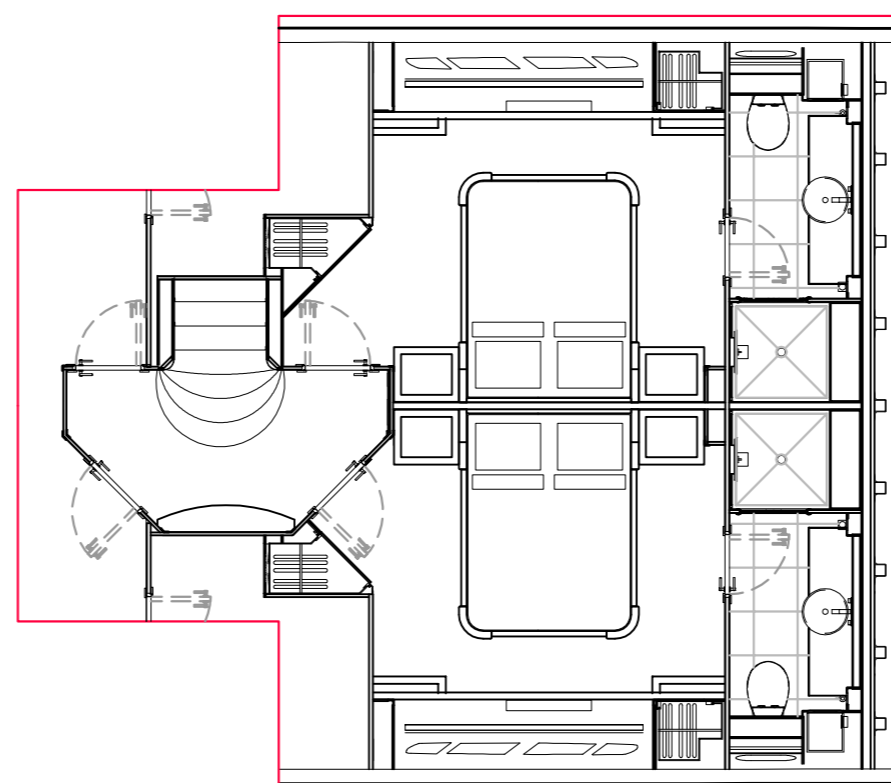
LOWER DECK OPTION Port & stbd double guest cabins
