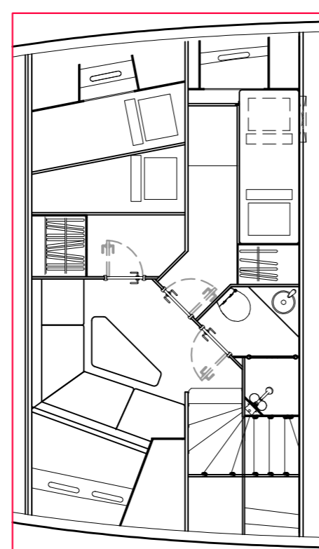
LOWER DECK OPTION Two cabin crew arrangement
