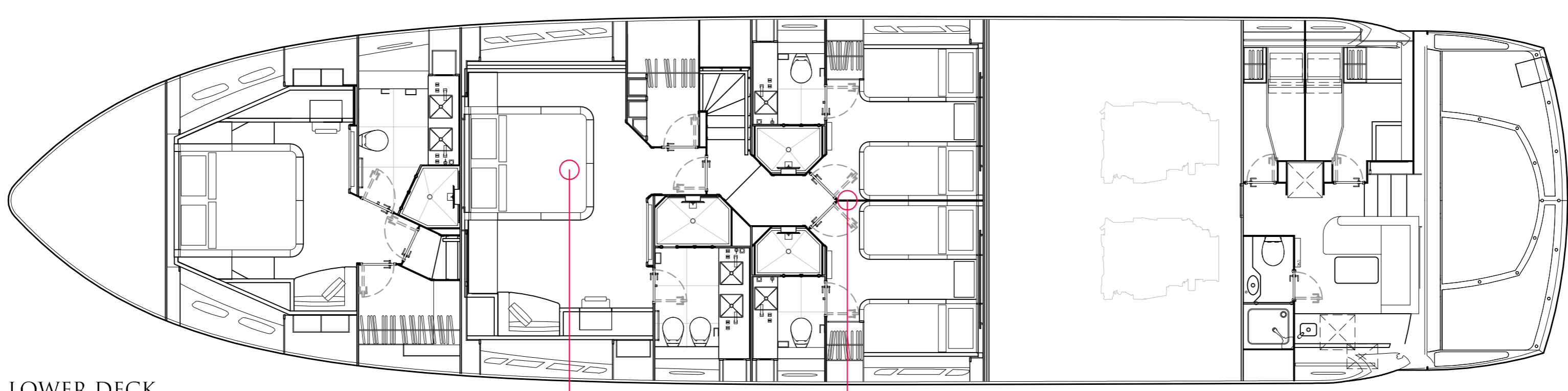
LOWER DECK
