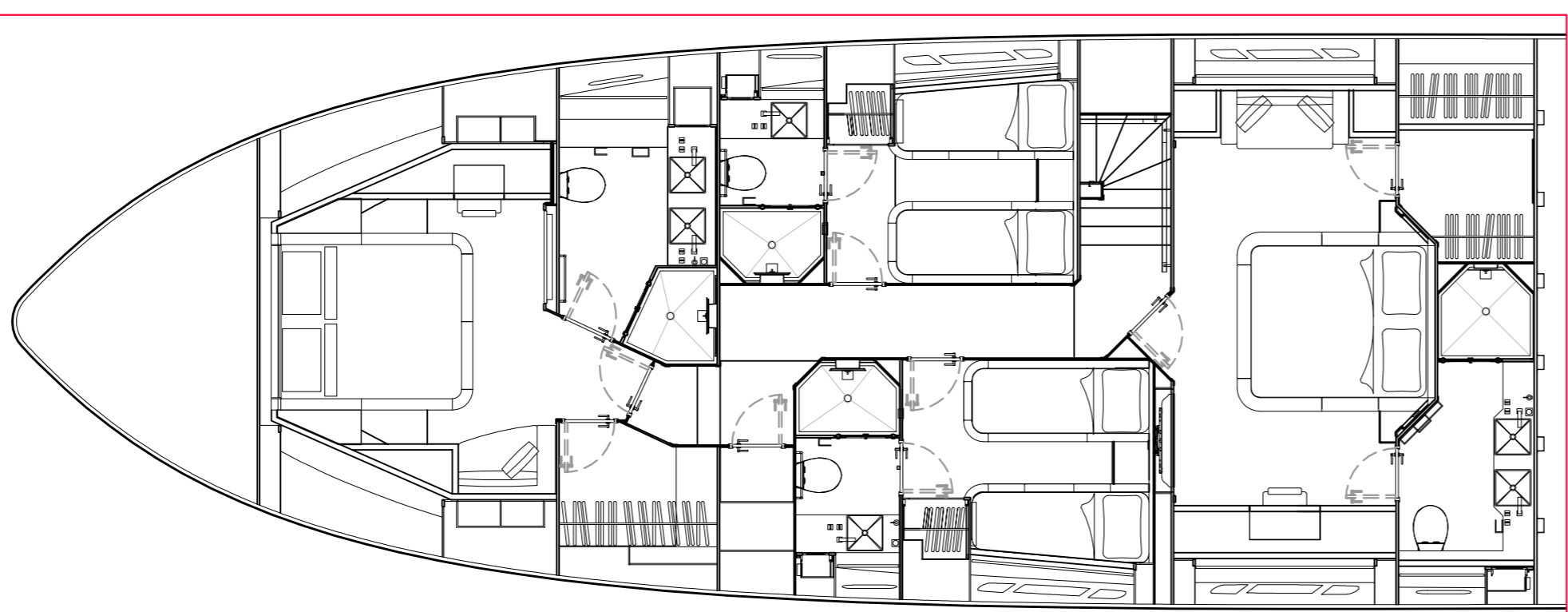
Optional single lower deck accommodation access
