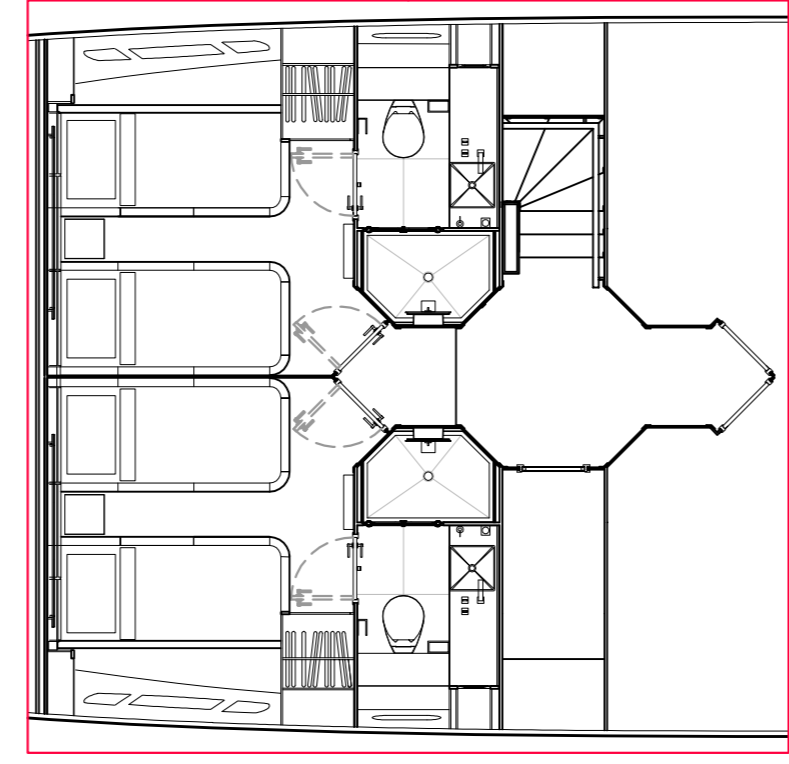
Optional Midship port & starboard Twin Guest Cabins
