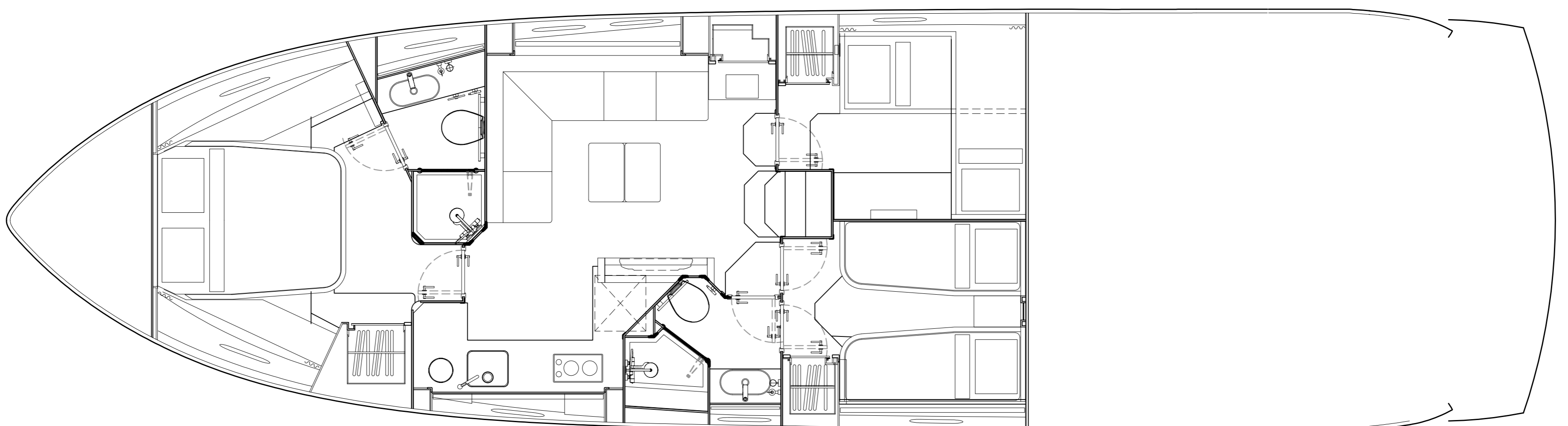
LOWER DECK
