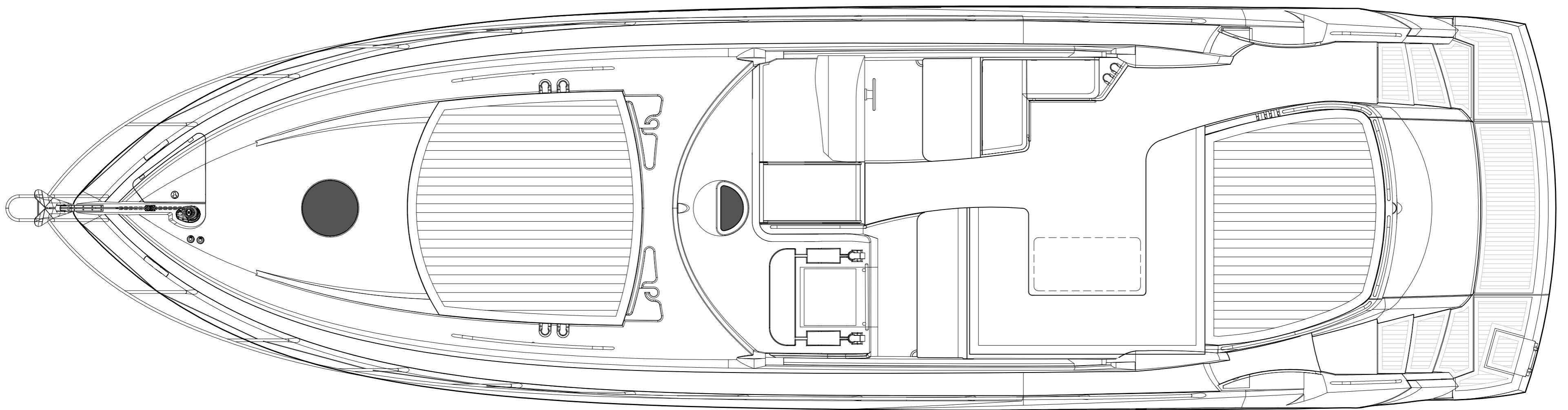
MAIN DECK
