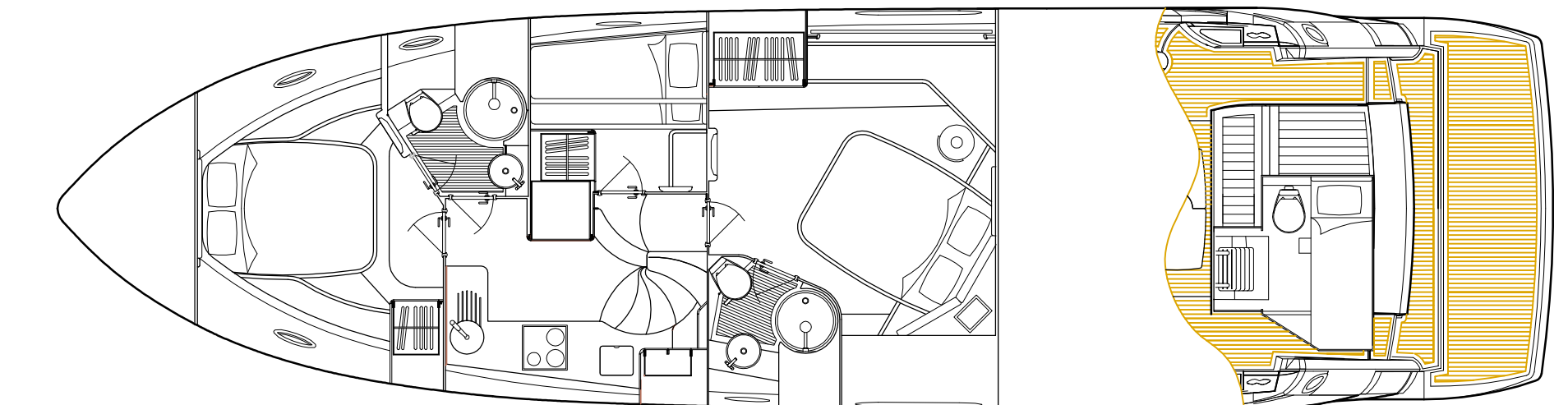
Lower Deck
