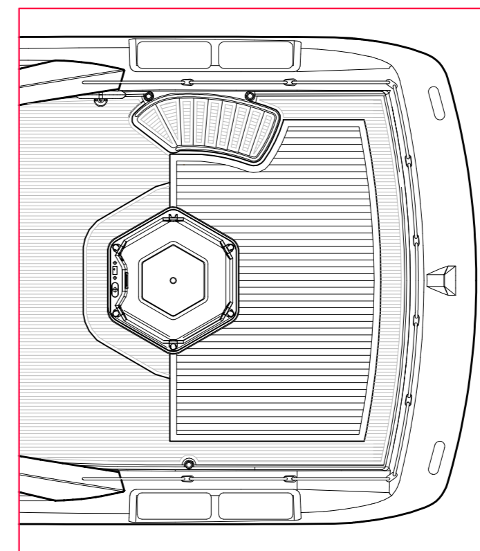
FLYBRIDGE OPTION Spa tub with sunpad
