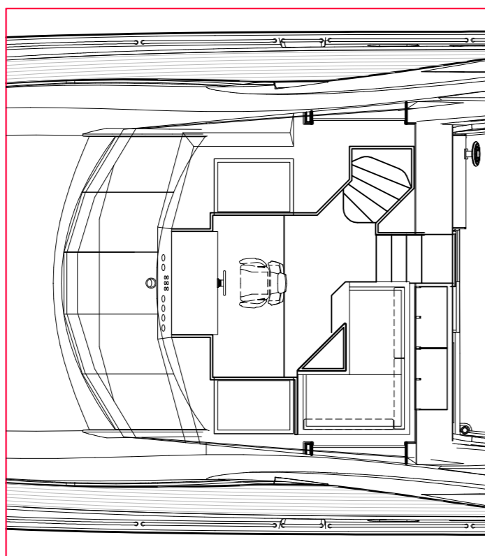
WHEELHOUSE
