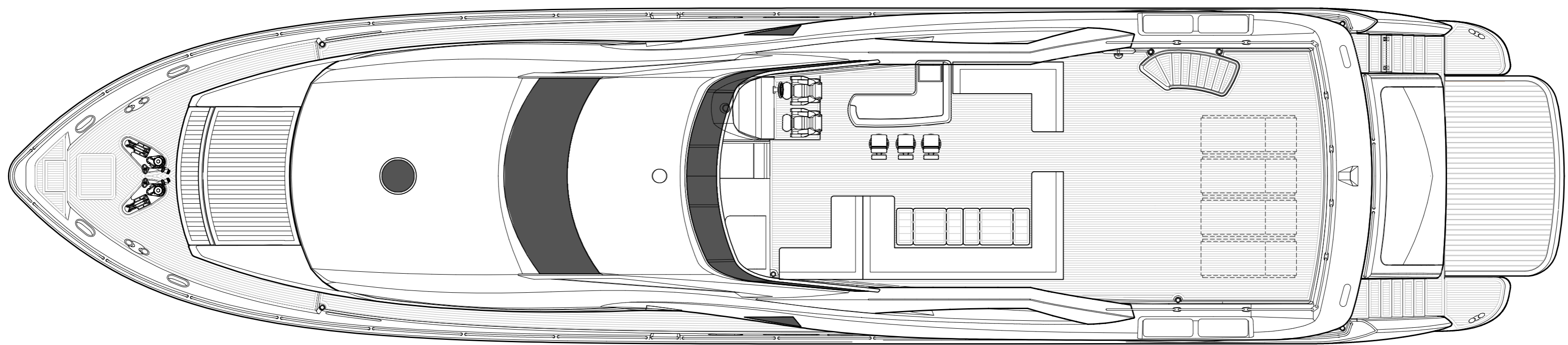
FLYBRIDGE Shown with optional teak decking
