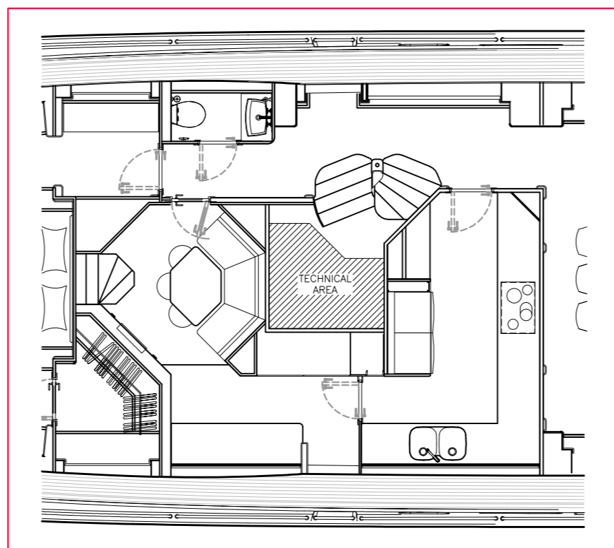
MAIN DECK OPTION Crew mess accessed from main deck lobby & stbd side entrance to galley
