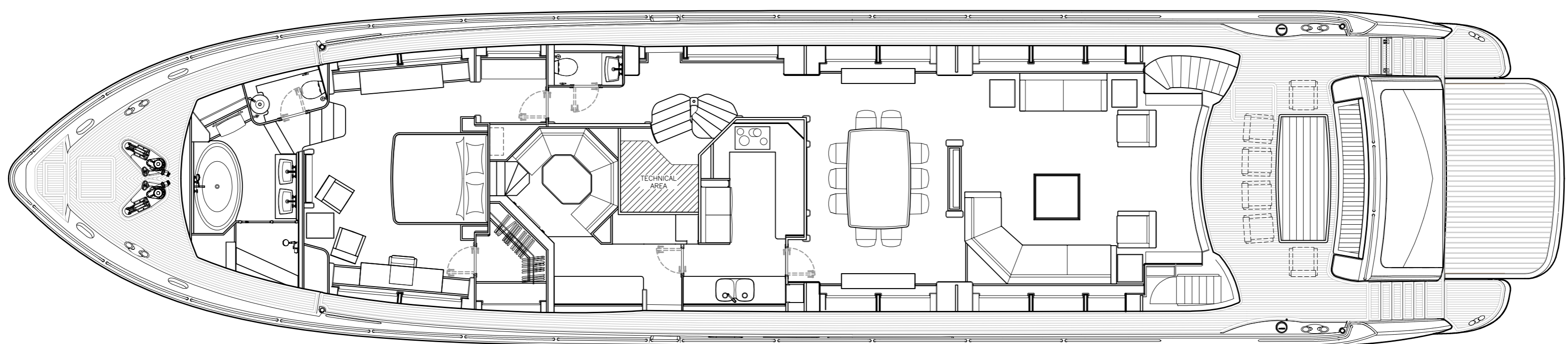
MAIN DECK
