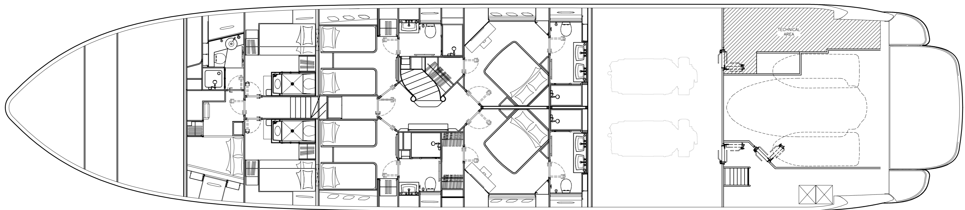
LOWER DECK
