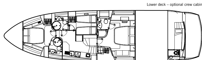
Lower deck – optional crew cabin
